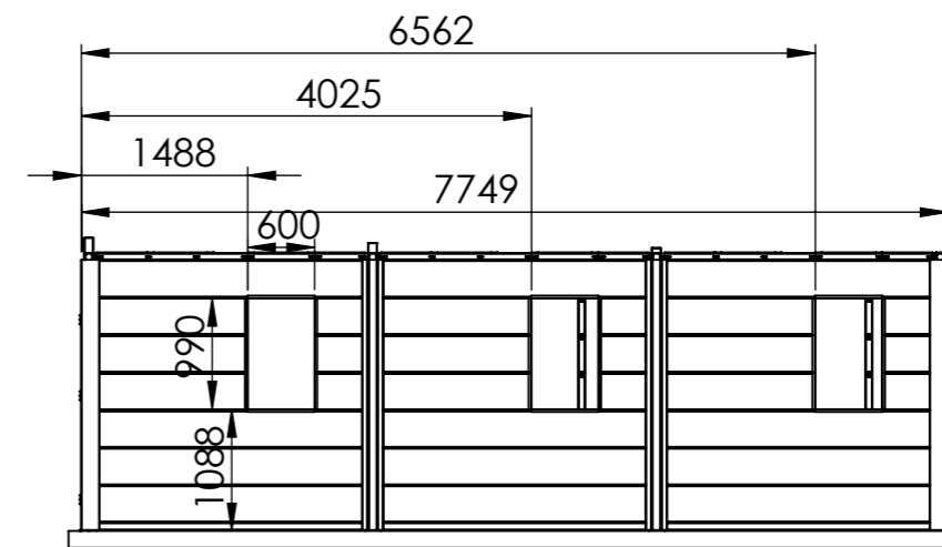
SECTION L-L SCALE 1 : 75
