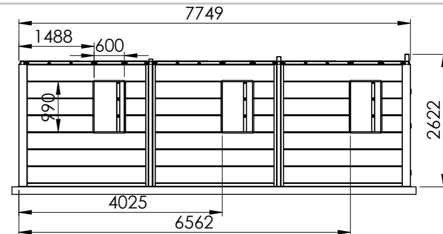
SECTION K-K SCALE 1 : 75
